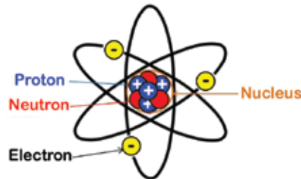
Lithium Atom
